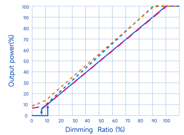
Output Power Vs. Dimming
